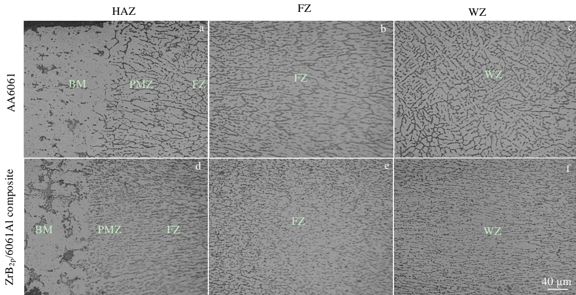
图 9 6061Al 合金和 ZrB_{2p}/6061Al 复合材料在 3.6 kW 和 2.4 m/min 下的焊接接头光学显微组织 Fig.9 OM microstructures of weld joints for 6061Al alloy and ZrB_{2p}/6061Al composite at power of 3.6 kW and welding speed of 2.4 m/min
