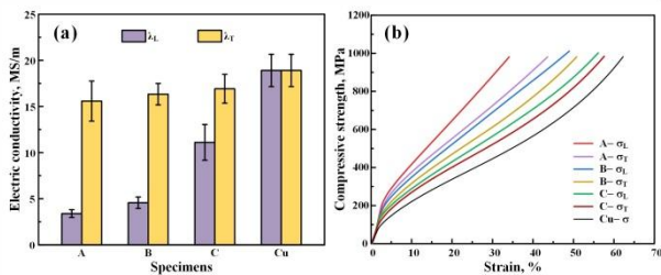
图 7 复合材料的 (a) 导电率 ( \lambda ) 和 (b) 抗压应力-应变曲线 Fig.7 (a) The electrical conductivity ( \lambda ) and (b) the compressive strength-strain curves of the composites
