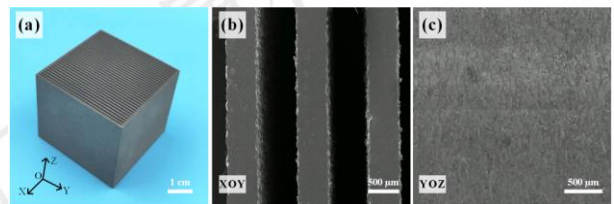
图 2B-316L 骨架的 (a) 宏观形貌，(b) 横截面，(c) 纵界面 Fig.2 (a) Macroscopic morphology, (b) cross-sectional structure and (c) longitudinal structure of the B-316L frameworks
