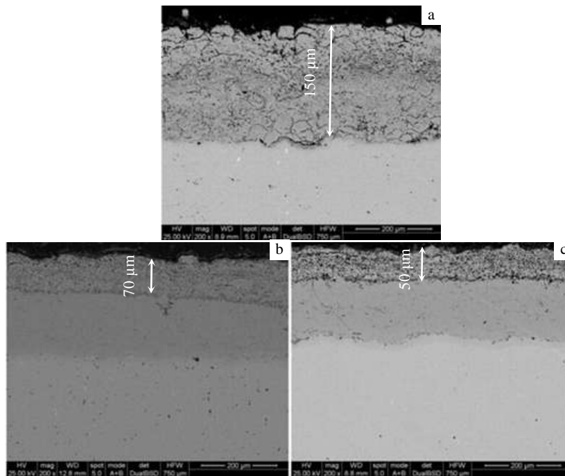
Fig.4 SEM micrographs of coatings after 150 h hot corrosion at 800 °C: (a) 0wt%Si, (b) 2wt%Si, and (c) 5wt%Si
