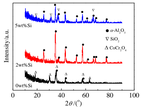
Fig.3 Small-angle XRD patterns of alloy powders after 300 h oxidation at 1000 °C
