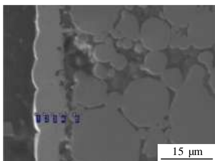
Fig.3 Typical Pd and Ag distribution obtained in the deposits by codeposition
