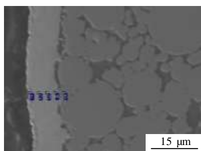
Fig.8 Typical Pd and Ag distribution obtained in the deposits prepared by sequential deposition
