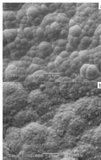
Fig.5 Deposition characteristics of Pd electroless deposits (a) and Ag electroless deposits by two-layer sequential deposits (b)
