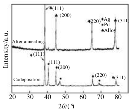
Fig.4 XRD patterns of the samples prepared by co-deposition and after annealing at 600 °C for 10 h in Ar gas
