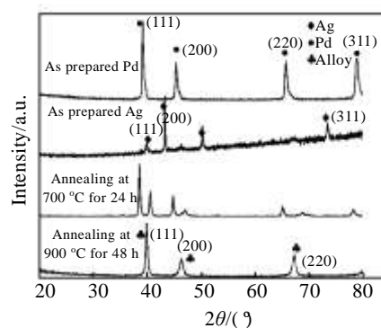
Fig.6 XRD patterns of the samples prepared with two-layer sequential deposition
