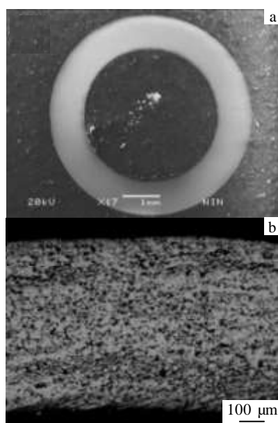
Fig.1 SEM image (a) and optical morphology(b) of the PSS
