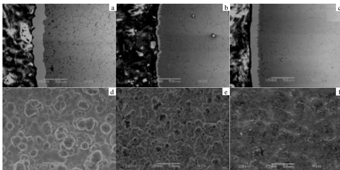
Fig.7 Deposition characteristics of Pd electroless deposits (a, d) Ag electroless deposits (b, e), and sequential deposits (c, f)
