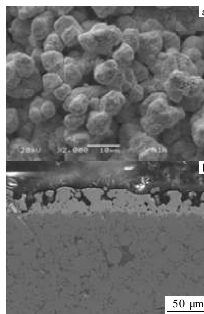
Fig.2 SEM images of Pd-Ag composite membranes by electroless codeposition (Pd/Ag=77/23): (a) top view and (b) cross-section view
