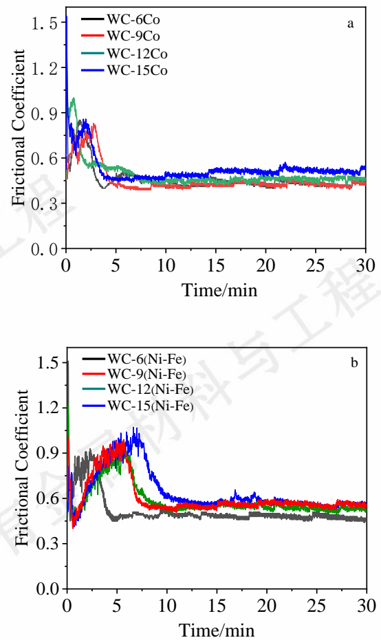
图 8 不同粘结相含量WC-Co和WC-Ni-Fe硬质合金摩擦磨损曲线 Fig.8 Friction wear curves of WC-Co and WC-Ni-Fe cemented carbides with different binder phase contents
