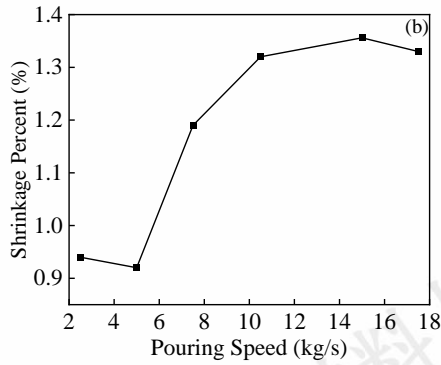
图9 (a) 6t Monel K-500 合金不同浇注速度真空感应锭缩孔云图； (b) 6t Monel K-500 合金真空感应锭缩孔缺陷随浇注速度变化图 Fig.9: (a) Shrinkage defect contour maps of 6-ton Monel K-500 alloy vacuum induction ingots at different pouring speeds; (b) Variation of shrinkage defects in 6-ton Monel K-500 Alloy vacuum induction ingots with pouring speed
