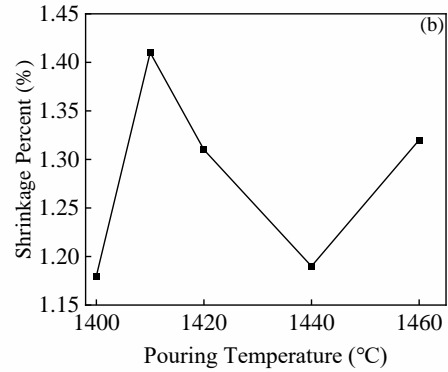
图10 (a) 6t Monel k-500 合金不同浇注温度真空感应锭缩孔云图； (b) 6t Monel k-500 合金真空感应锭缩孔缺陷随浇注温度变化图 Fig.10: (a) Shrinkage defect contour maps of 6-ton Monel K-500 alloy vacuum induction ingots at different pouring temperatures; (b) Variation of shrinkage defects in 6-ton Monel K-500 alloy vacuum induction ingots with pouring temperature
